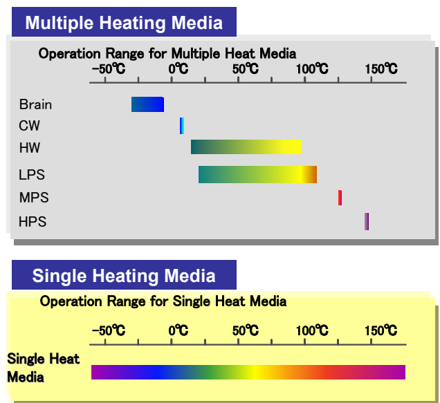
Fig. 1. Operation Range for Heating Media
