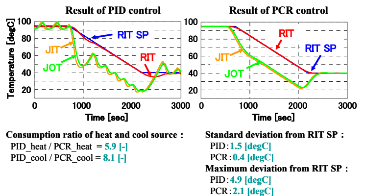
Fig.6. Temperature Control for Crystallization (PID vs PCR)
